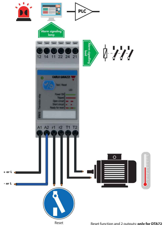
Reset function and 2 outputs: only for DTA72
